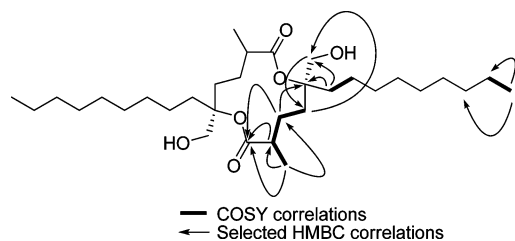
Figure 1. Selected 2D NMR correlations for malyngolide dimer ( 1 ).
